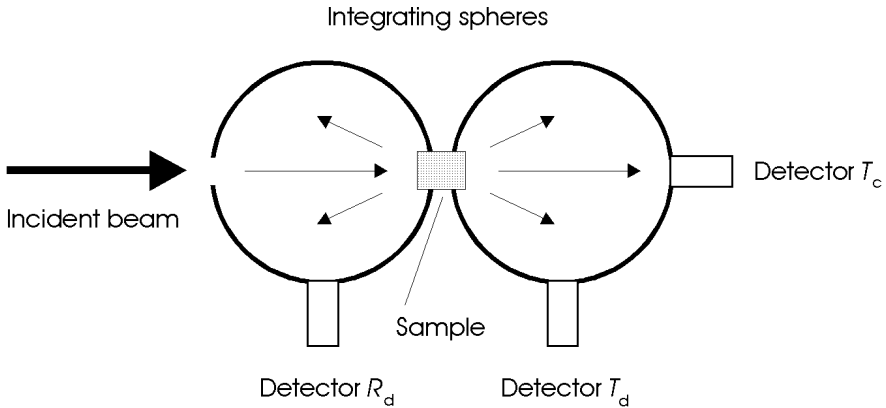
Fig. 2.16. Double-integrating sphere geometry for the simultaneous measurement of different optical tissue properties. The detectors measure the transmitted coherent intensity ( T_c ), the transmitted diffuse intensity ( T_d ), and the reflected diffuse intensity ( R_d )
