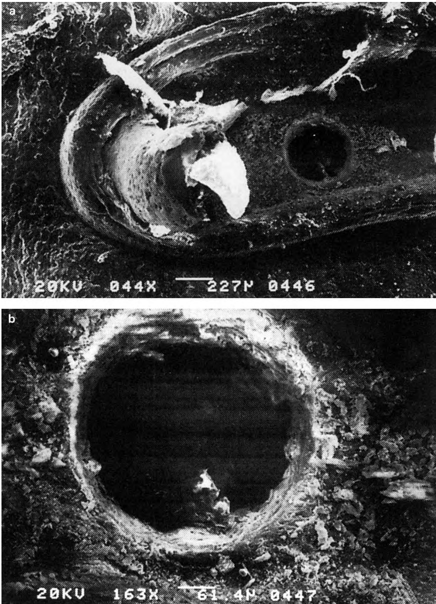
Fig. 4.70. (a) Stapedotomy performed with five pulses from an Er:YAG laser (pulse duration: 200\ \mu\text{s} , fluence: 10\ \text{J}/\text{cm}^2 ). (b) Enlargement of the perforation. Reproduced from Frenz et al. (1994) by permission. © 1994 Verlag Huber AG
