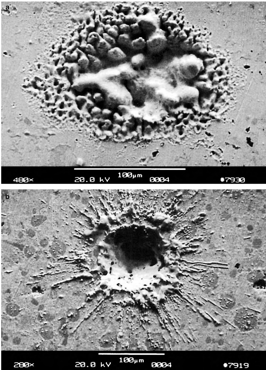
Fig. 4.40. (a) Removal of amalgam with a Nd:YLF laser (pulse duration: 30 ps, pulse energy: 0.5 mJ). (b) Removal of amalgam with an Er:YAG laser (pulse duration: 90 μs, pulse energy: 100 mJ)
