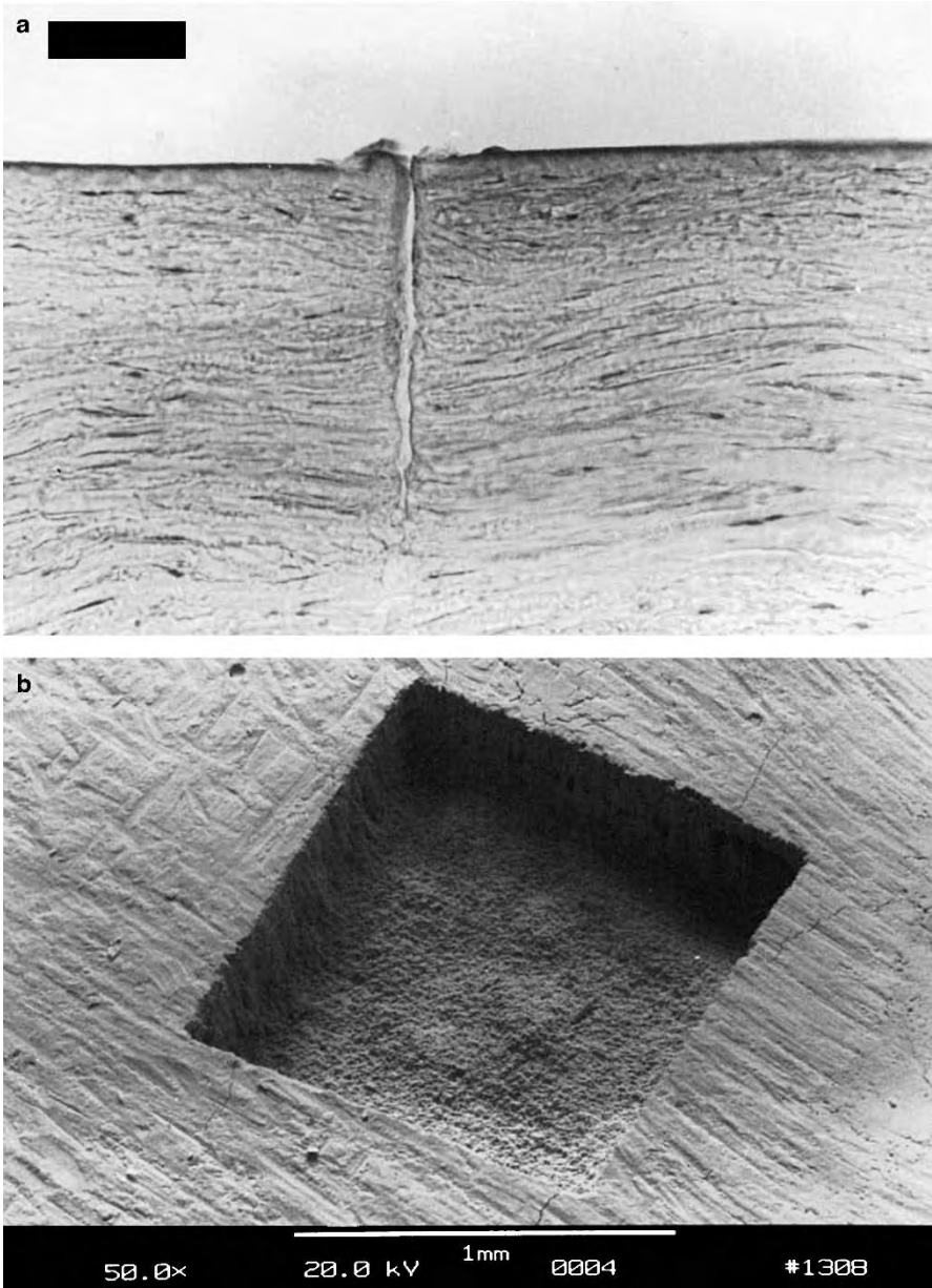
Fig. 3.41. (a) Excision in a human cornea achieved with a picosecond Nd:YLF laser (pulse duration: 30 ps, pulse energy: 200 \mu J, bar: 50 \mu m). (b) Human tooth exposed to 16 000 pulses from a picosecond Nd:YLF laser (pulse duration: 30 ps, pulse energy: 1 mJ, pattern size: 1 \times 1 mm 2 ). Superficial cracking occurred as an artefact during the preparation for electron microscopy
