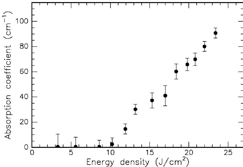
Fig. 3.44. Absorption of laser plasmas induced in distilled water by a Nd:YLF laser (wavelength: 1.053 \mu\text{m} , pulse duration: 30 ps). Unpublished data
