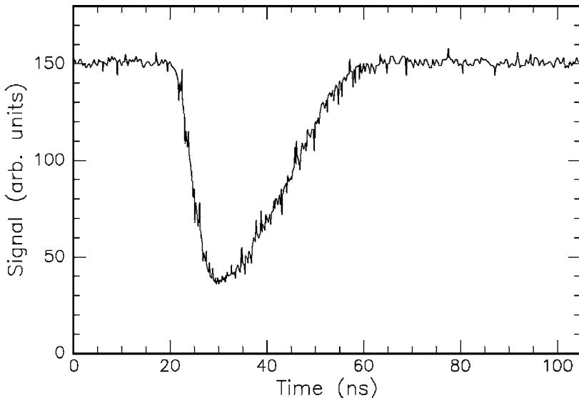
Fig. 3.67. Signal from a helium–neon laser serving as a detector for a shock wave generated in water by a Nd:YLF laser (pulse duration: 30 ps, pulse energy: 1 mJ)
